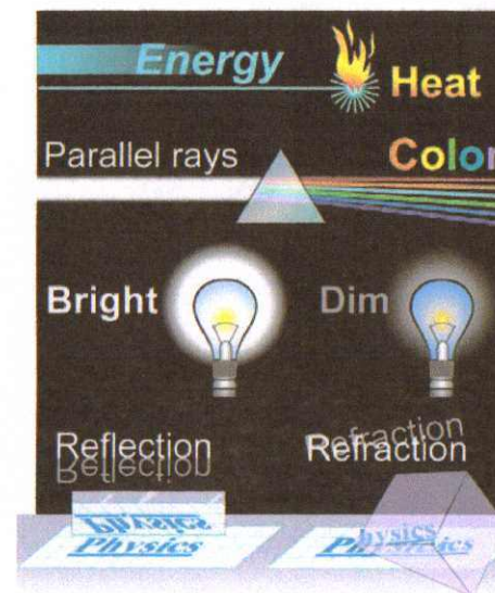
Figure 10.1: Some words and properties that are associated with light. What words do you use to describe light?
