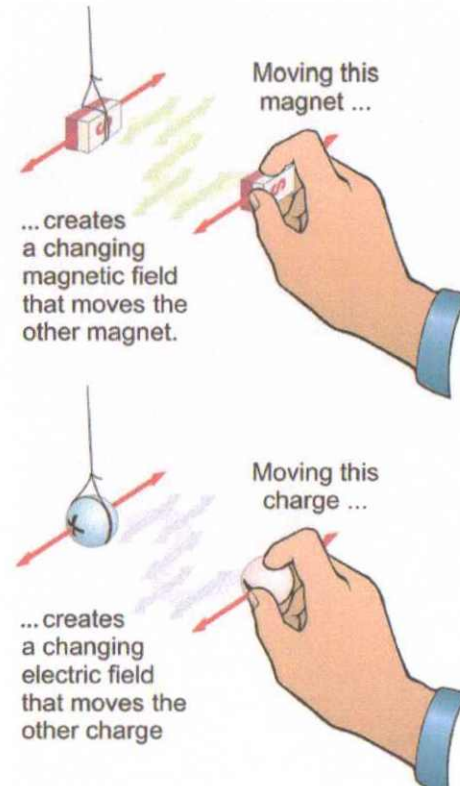
Figure 10.6: Magnets influence each other through the magnetic field. Charges influence each other through the electric field.
