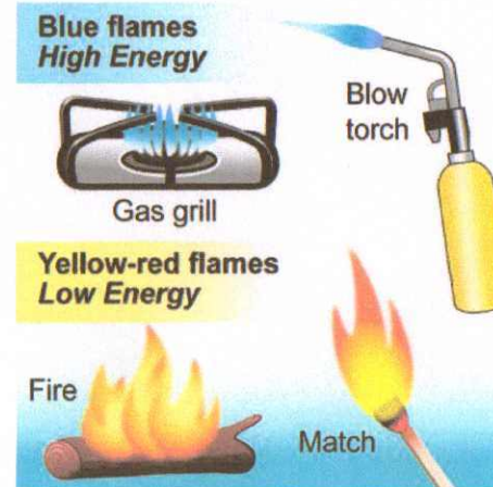
Figure 10.4: High-energy flames such as the ones from a gas grill produce blue light. Fire flames are lower energy and produce reddish-yellow light.
